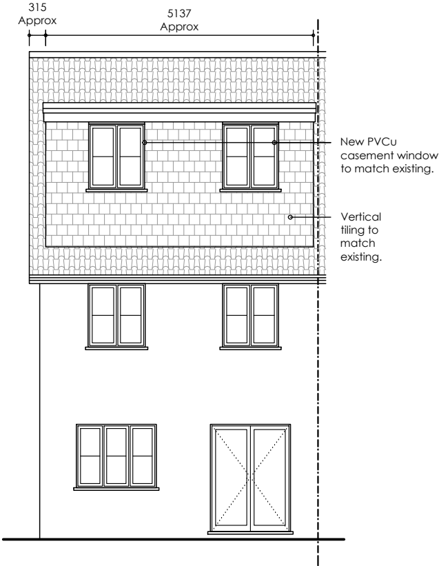
Proposed Rear Elevation Scale 1/100@A3
