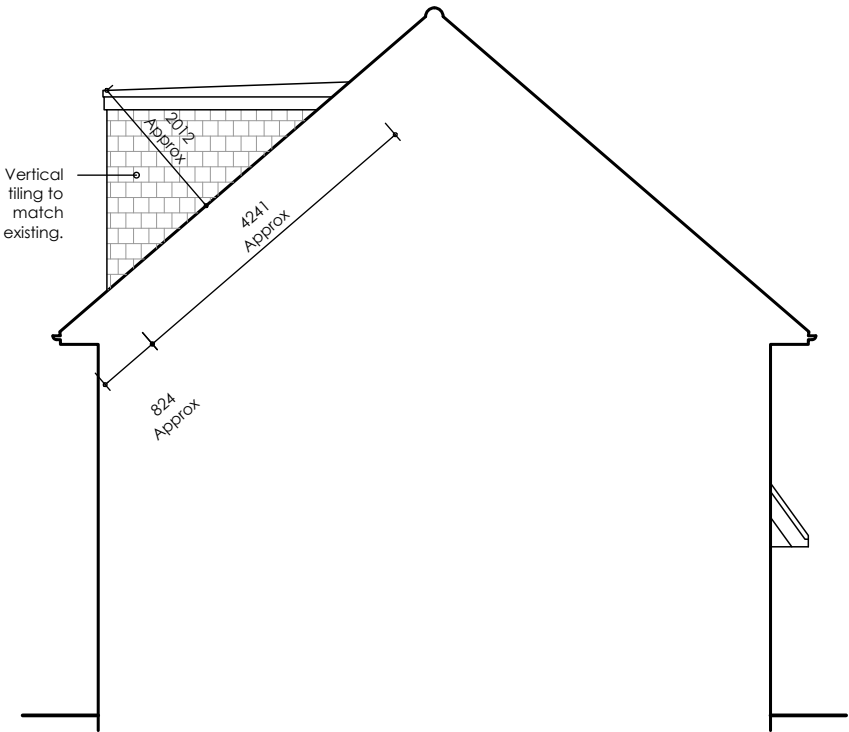
Proposed LHS Elevation Scale 1/100@A3
