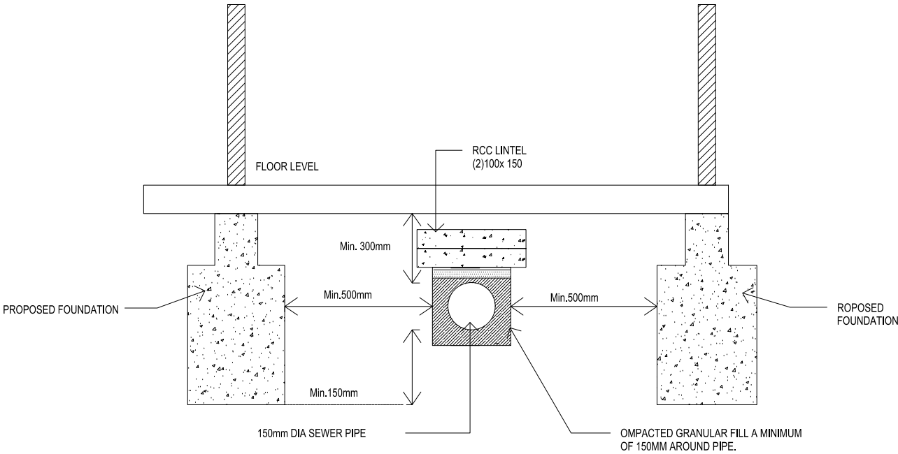
FOUNDATION DETAILS AND PIPEWORK PROTECTION
