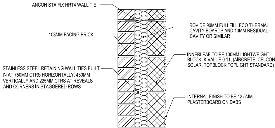
FULL FILL CAVITY WALL U-value 0.17 W/m 2 k
