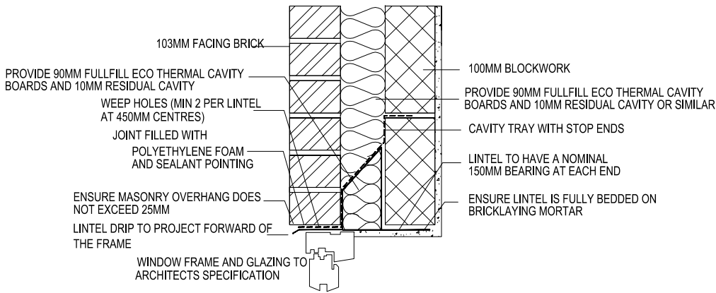
WINDOW HEAD AND LINTEL
