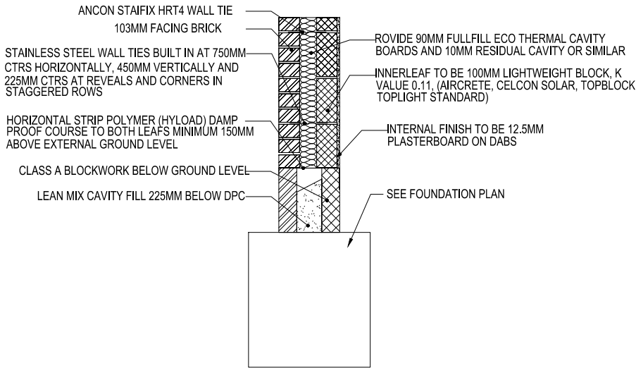
FULL FILL CAVITY WALL FOOTING U-value 0.18 W/m 2 k
