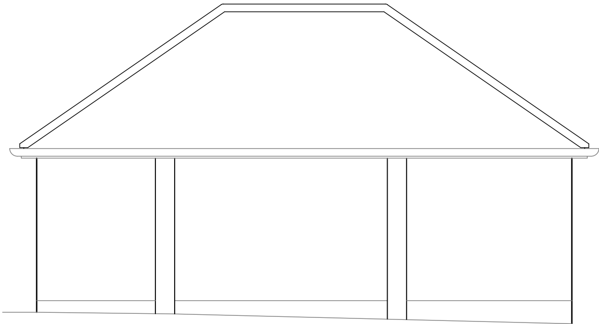
North Elevation - @ 1:50
