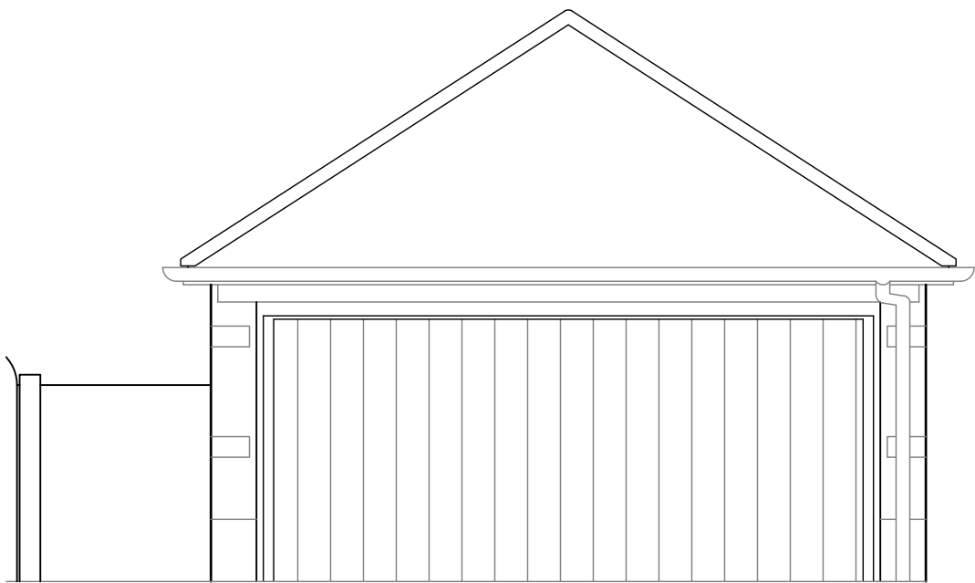
East Elevation - @ 1:50
