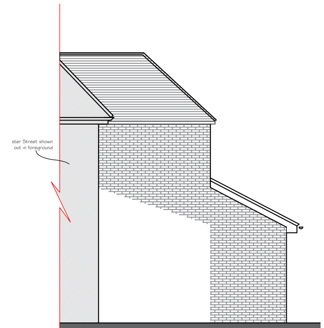
Proposed Side Elevation 1:100 @ A3
