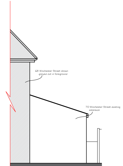
Existing Side Elevation 1:100 @ A3
