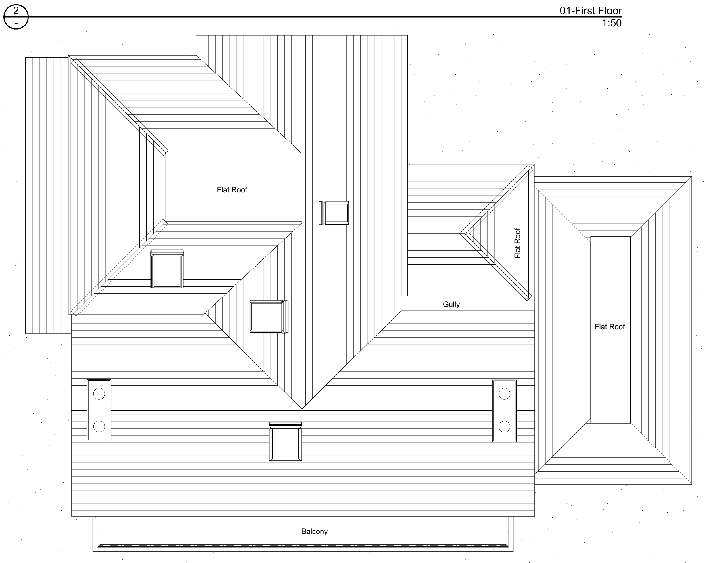
Roof 1:50
