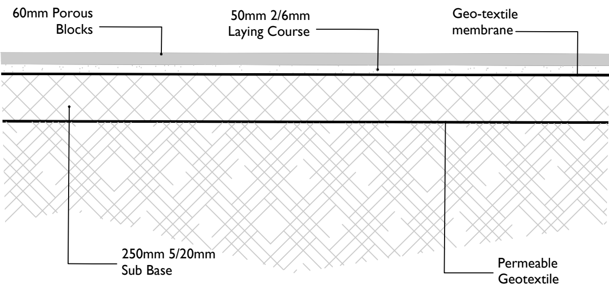
Porous Paved Area for Staff Overflow
