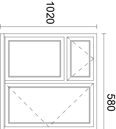
PROPOSED ELEVATION
