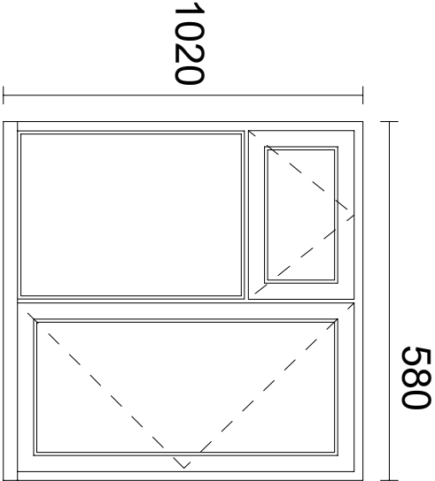
EXISTING ELEVATION
