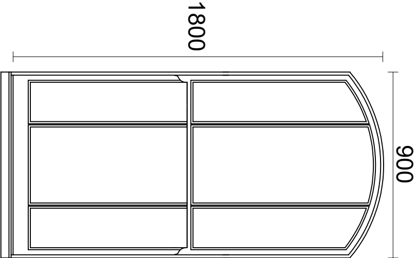
EXISTING ELEVATION
