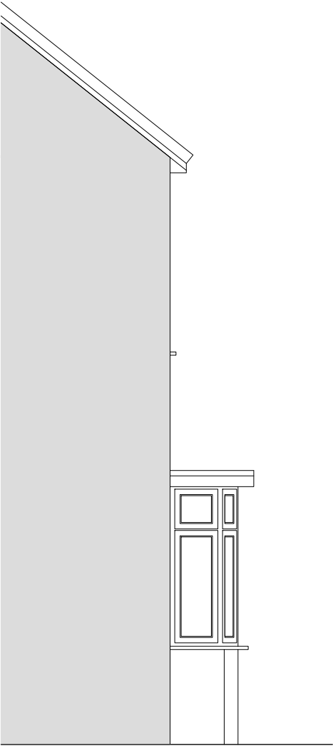
EXISTING LEFT ELEVATION Scale 1:50
