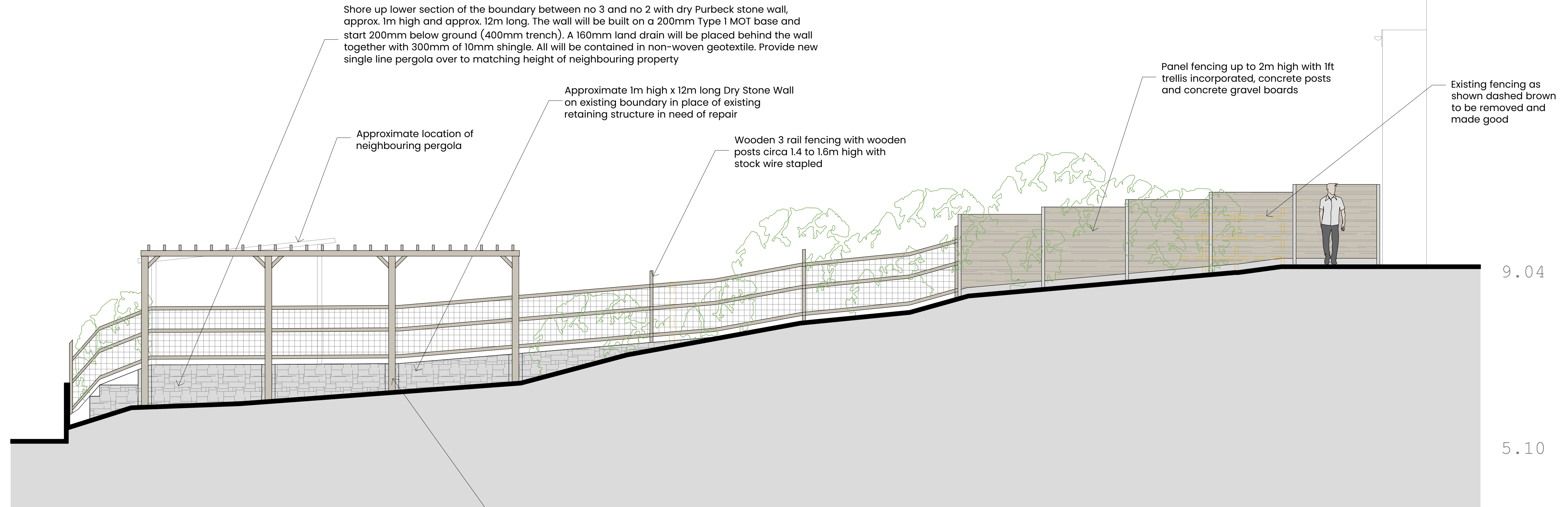
Southern Elevation
