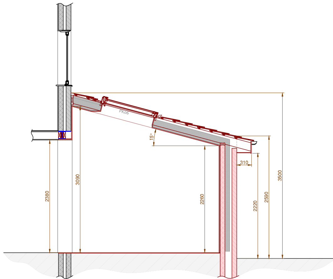
Proposed Section - New Extension
