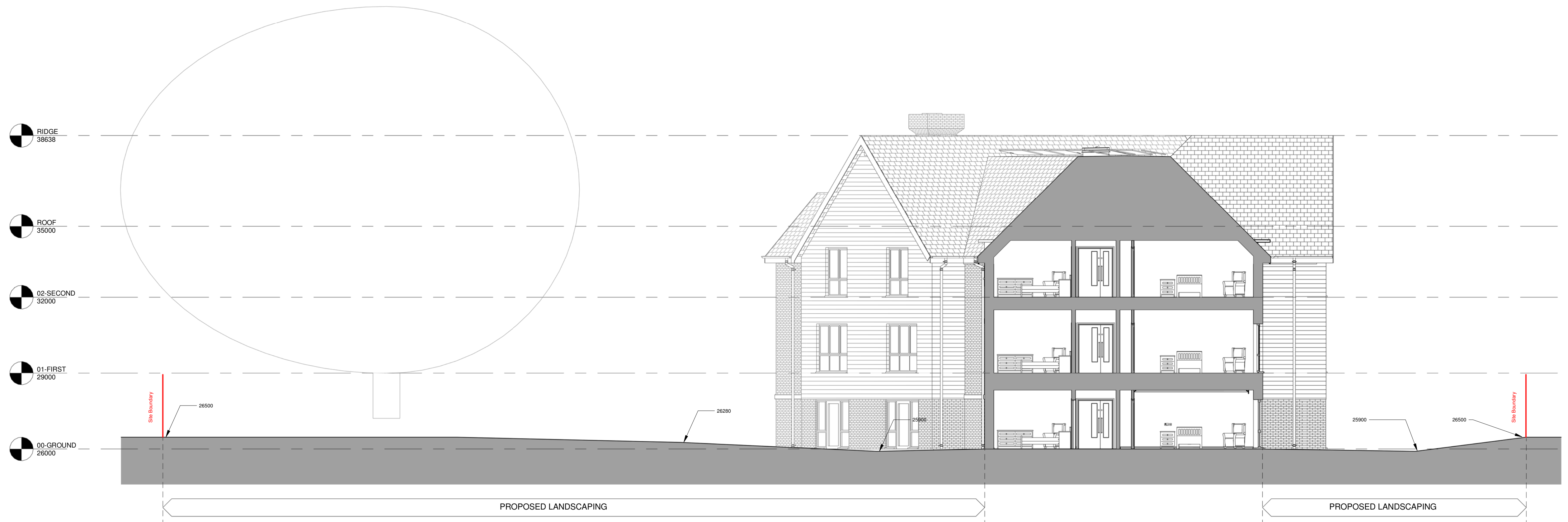
2 Proposed Site Section B-B 1 : 100
