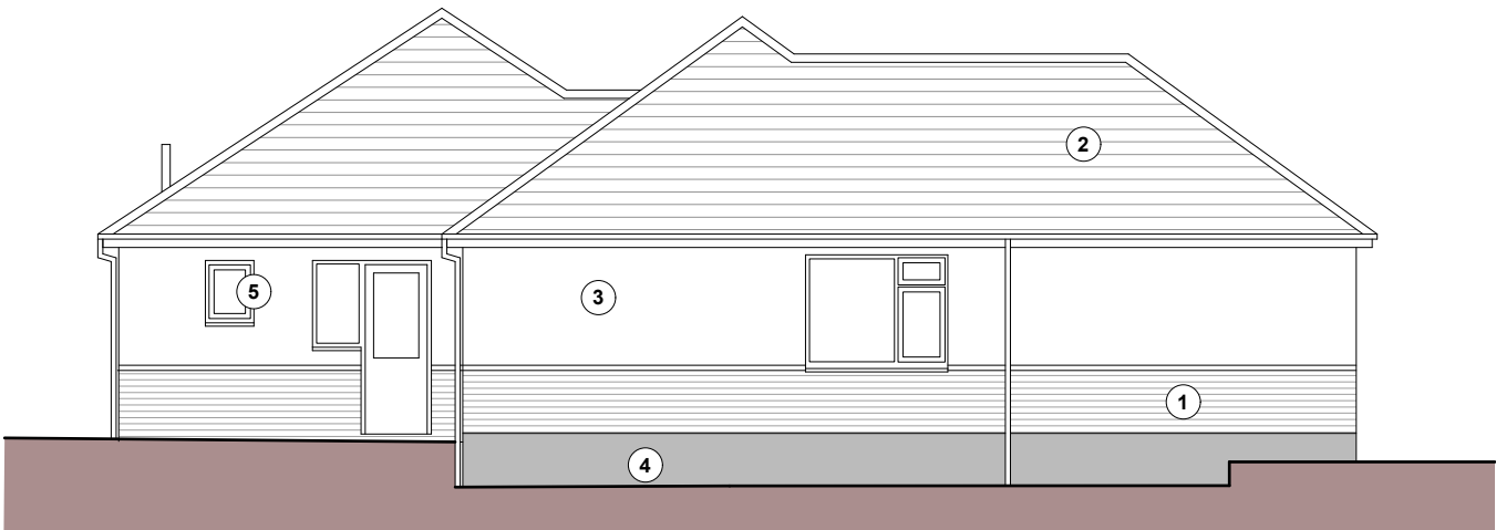
EXISTING NORTH-WEST ELEVATION Scale 1:100
