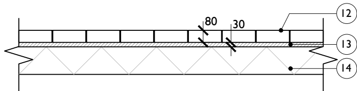
Tobermore Artro Paving Slate
