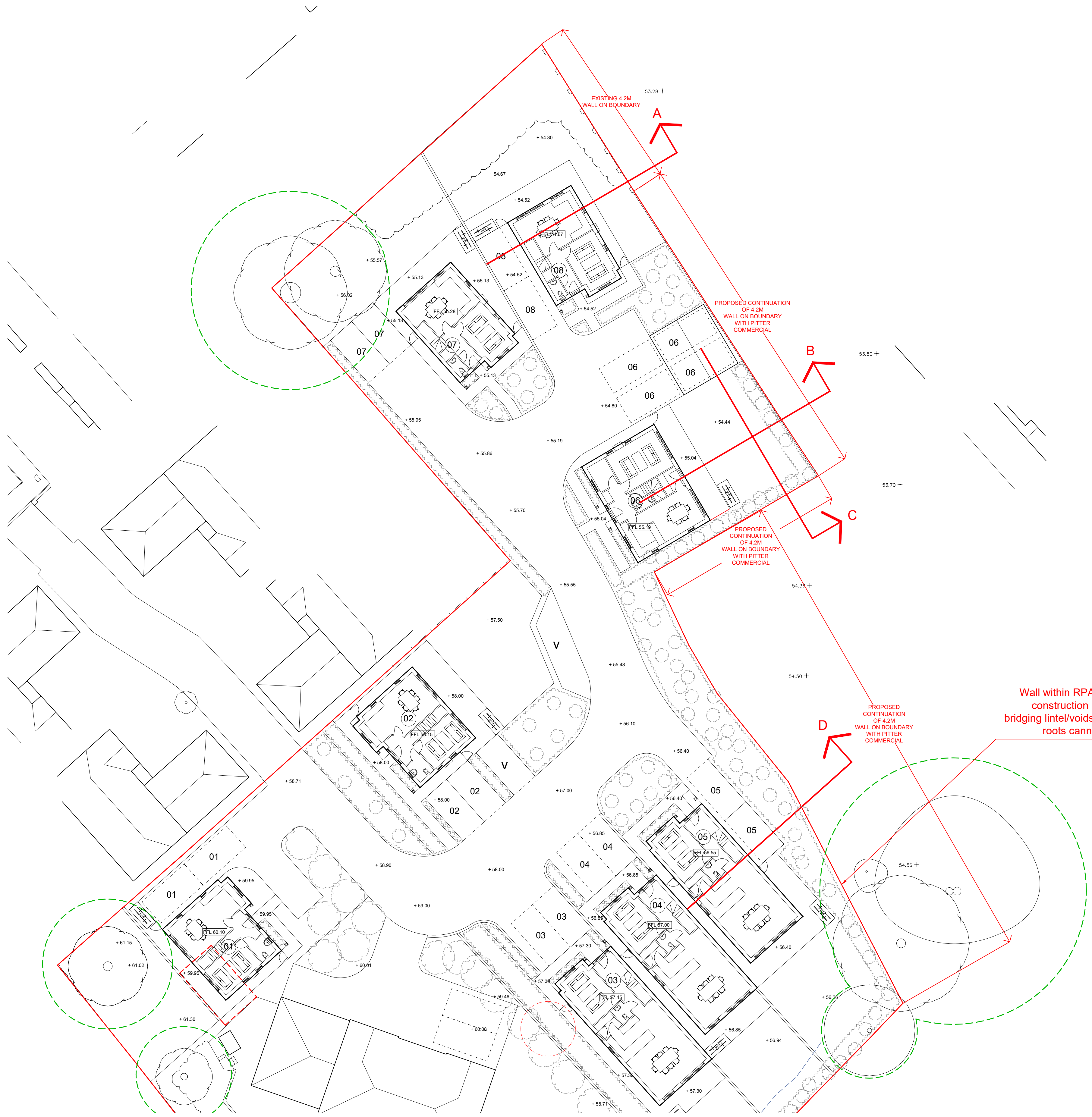
Site Layout / Section Reference
