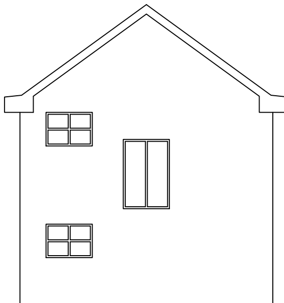
SIDE ELEVATION 01
