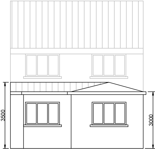
REAR ELEVATION
