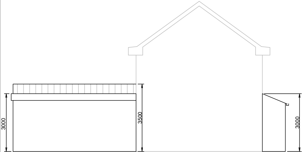
SIDE ELEVATION 02
