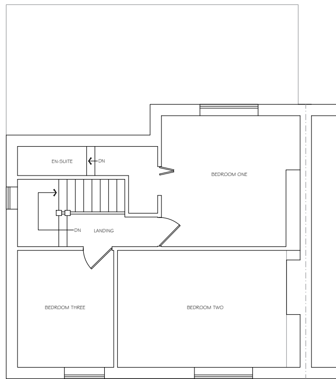
Existing First Floor Plan 1:100 @ A3
