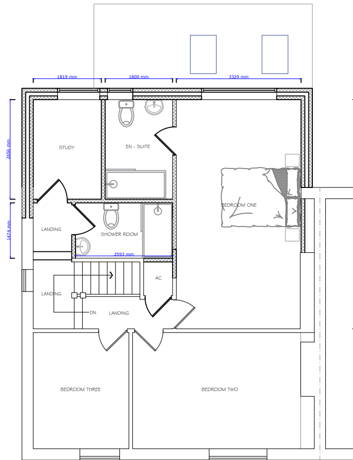
Proposed First Floor Plan 1:100 @ A3
