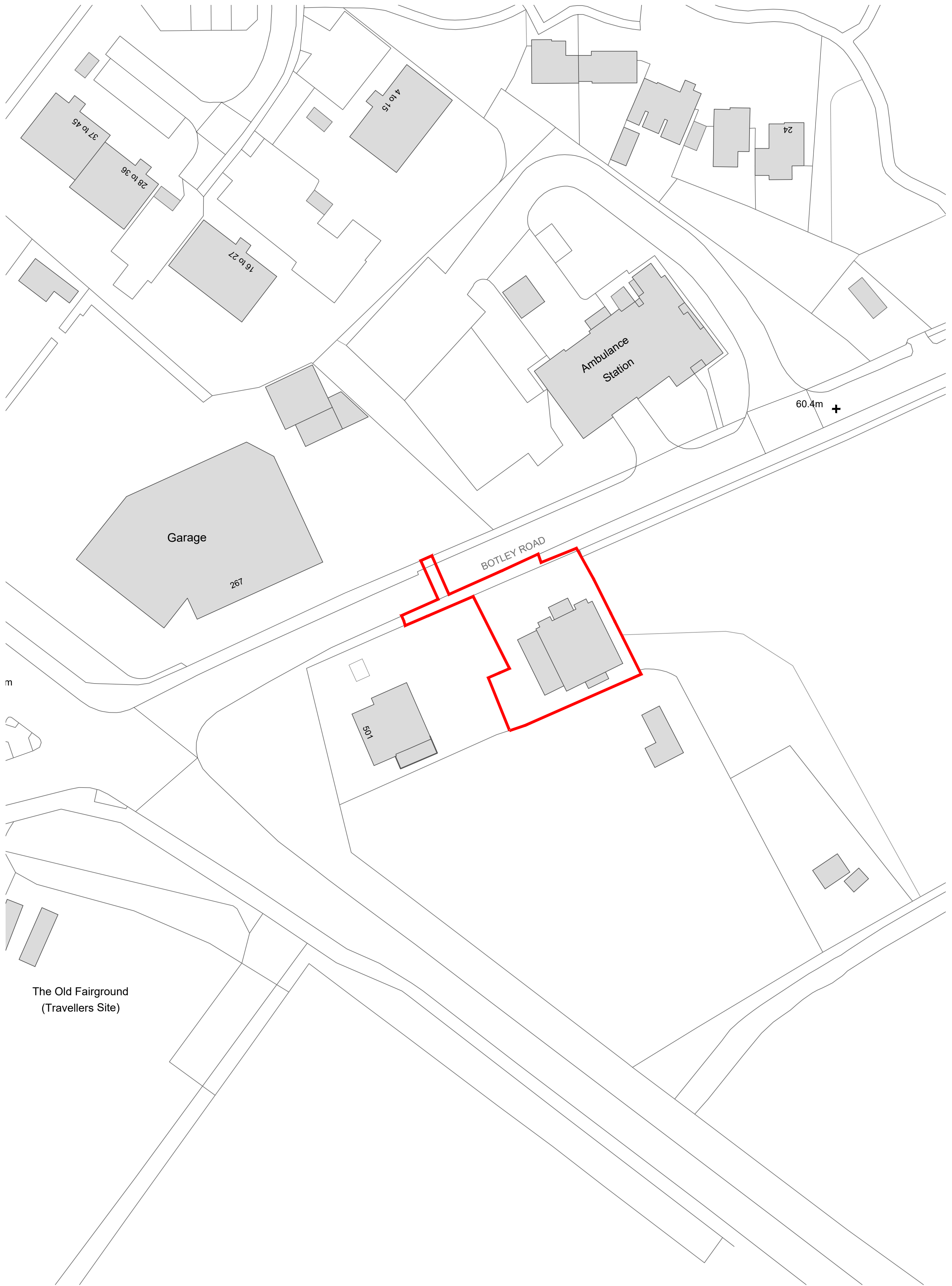
Block Plan Proposed at 1:500
