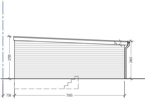
North Elevation
