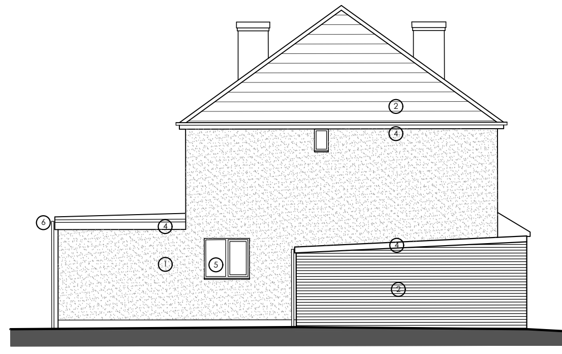
EAST ELEVATION
