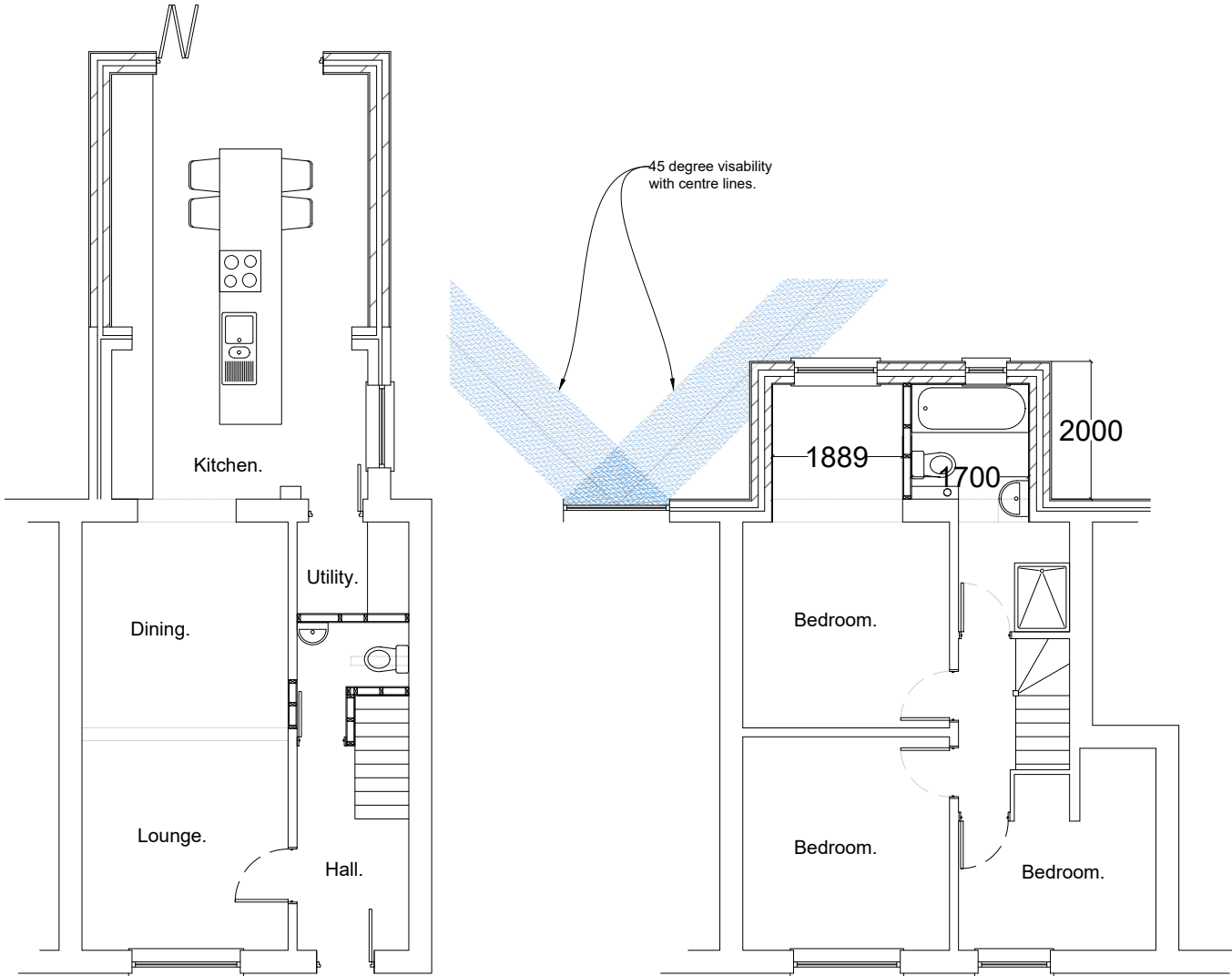
Ground Floor.
