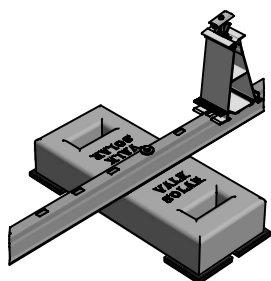
Mass blocks: Roof or field systems
