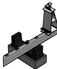
Elevation blocks: for gravel roofs
