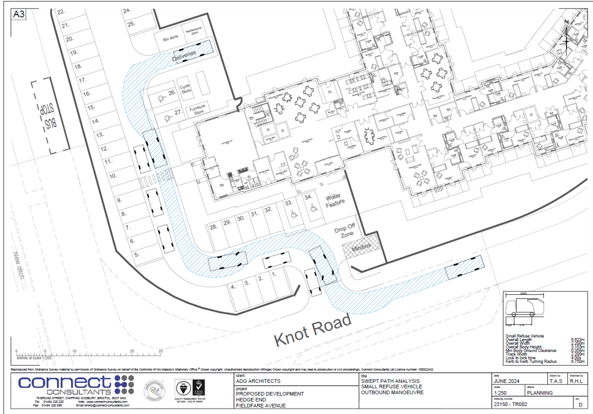
Figure 2: Transport Statement, dated June 2024, Appendix 3 - Swept Path Analysis, Small Refuse Vehicle, Outbound Manoeuvre
