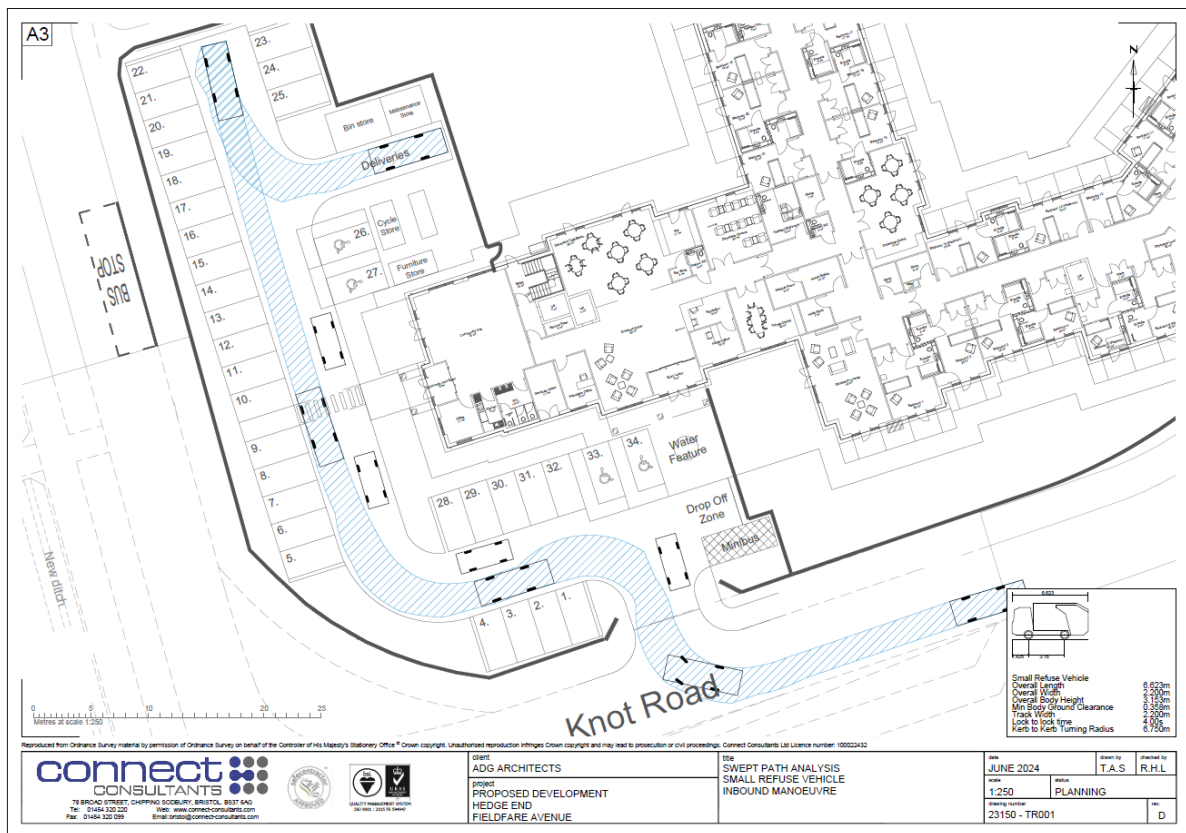
Figure 1: Transport Statement, dated June 2024, Appendix 3 - Swept Path Analysis, Small Refuse Vehicle, Inbound Manoeuvre
