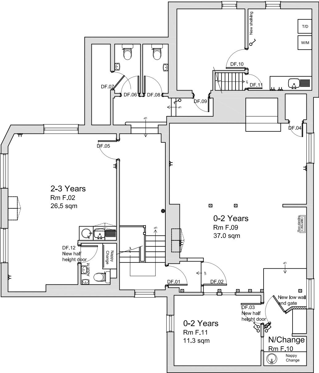
Proposed First Floor GA Plan
