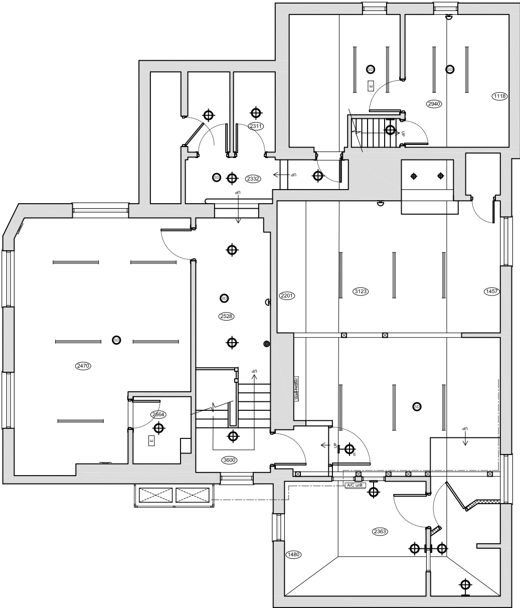
Proposed First Floor Reflected Ceiling Plan
