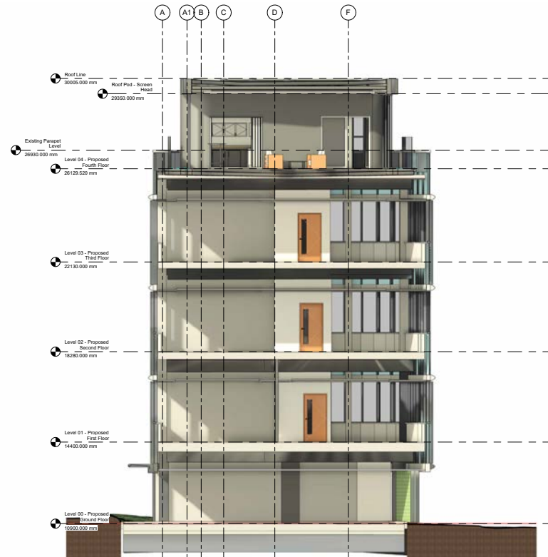
Proposed Cross Section 2
