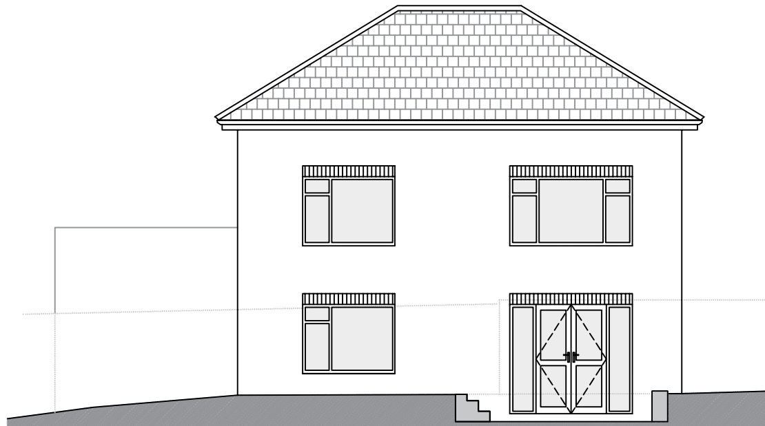
Proposed Rear Elevation 1:100 @ A3
