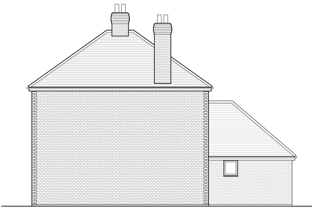
South-West (Side) Elevation - As Existing
