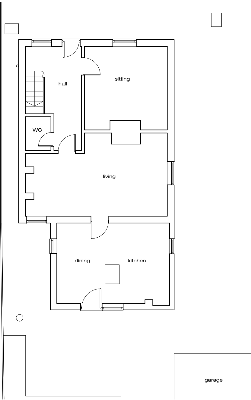
Ground Floor Plan - As Existing
