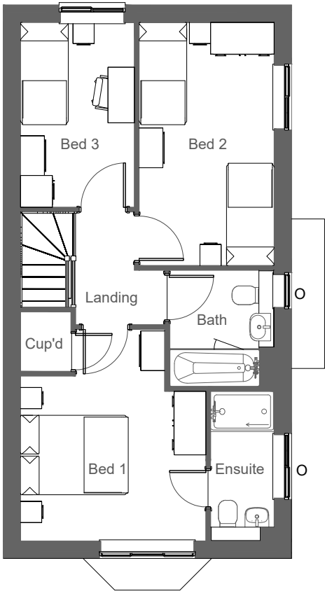
First Floor Plan O= Obscure glazed window.
