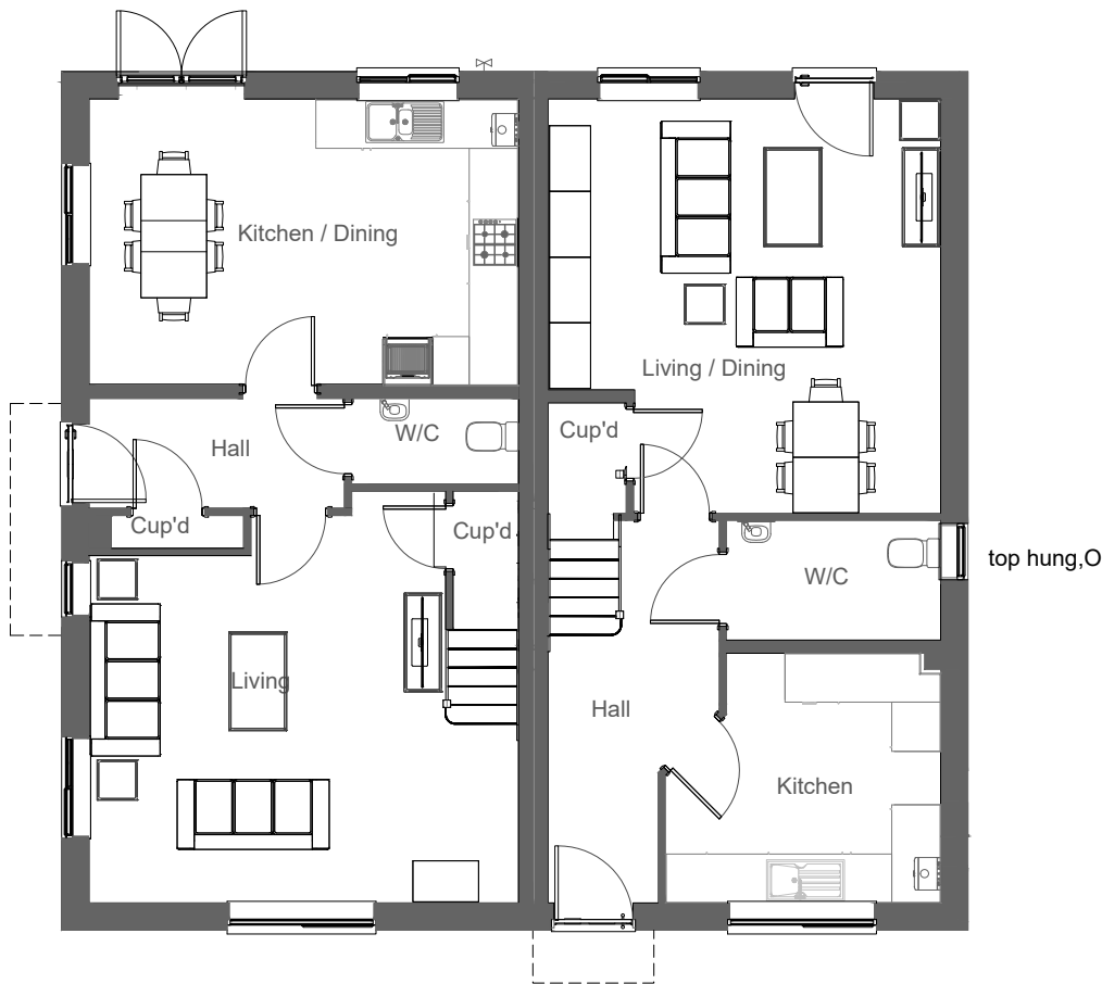
Ground Floor Plan O= Obscure glazed window.
