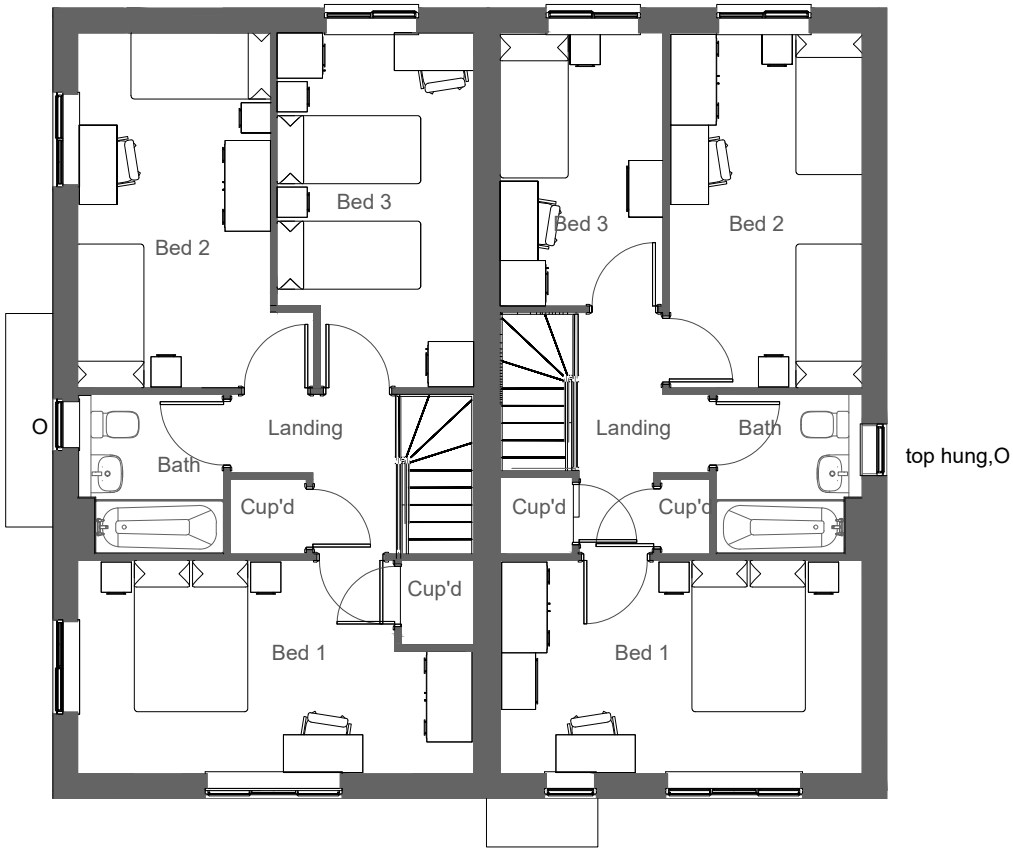
First Floor Plan O= Obscure glazed window.
