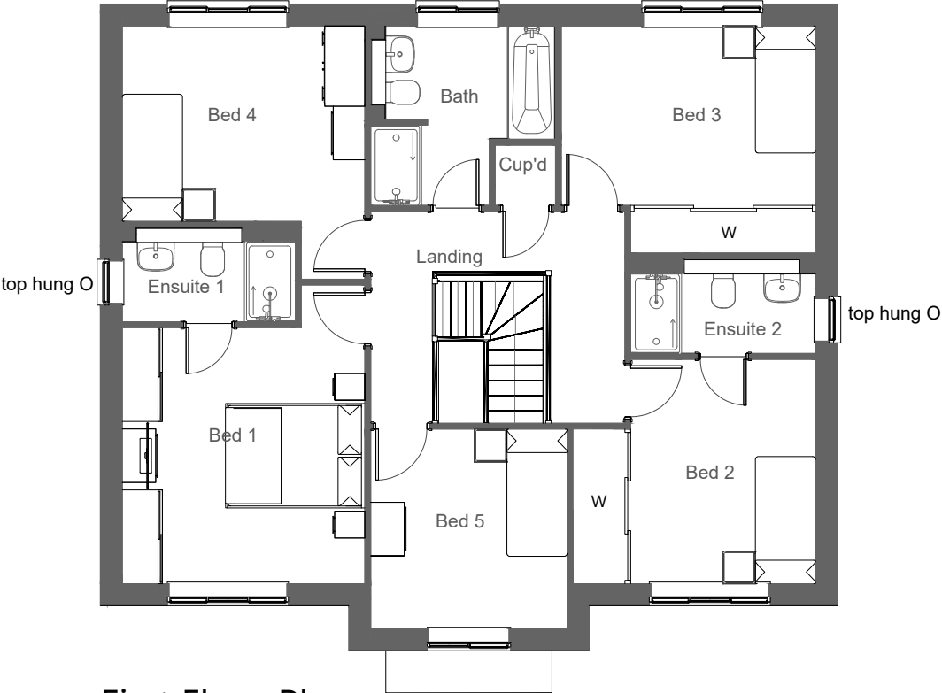
First Floor Plan O= Obscure glazed window.
