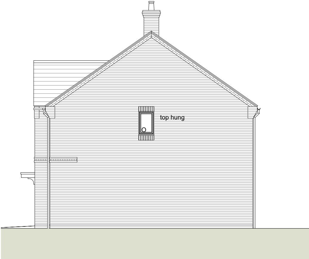
Side Elevation
