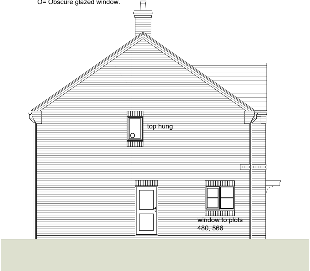
Side Elevation
