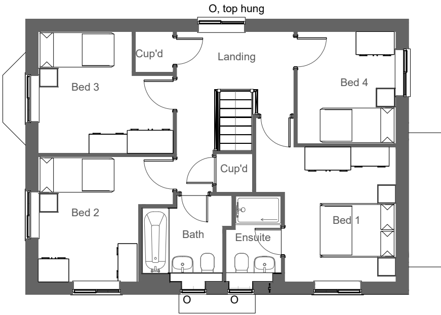
First Floor Plan O= Obscure glazed window.
