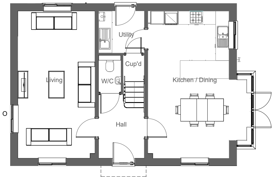
Ground Floor Plan O= Obscure glazed window.
