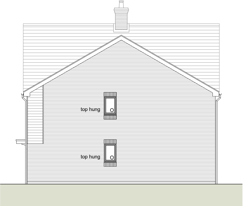
Side Elevation
