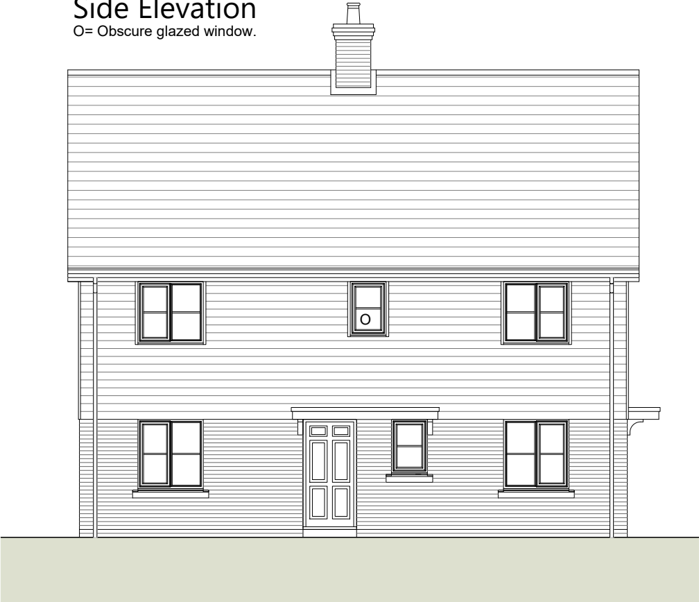
Side Elevation
