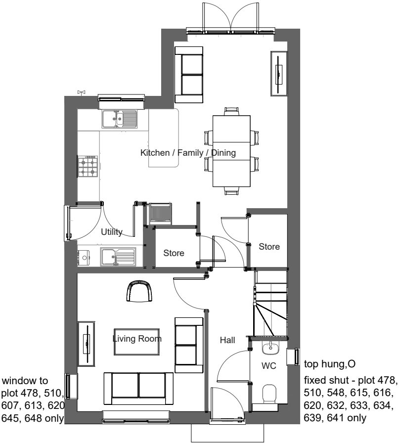
Ground Floor Plan O= Obscure glazed window.
