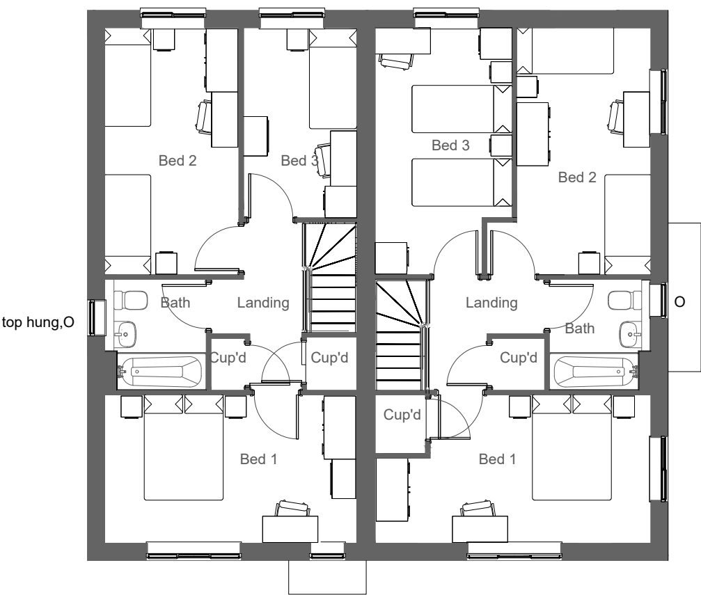
First Floor Plan O= Obscure glazed window.
