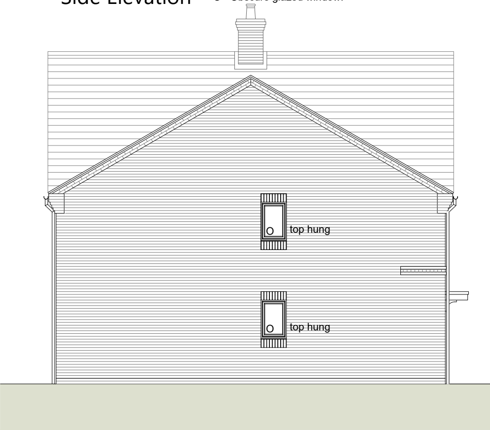
Side Elevation
