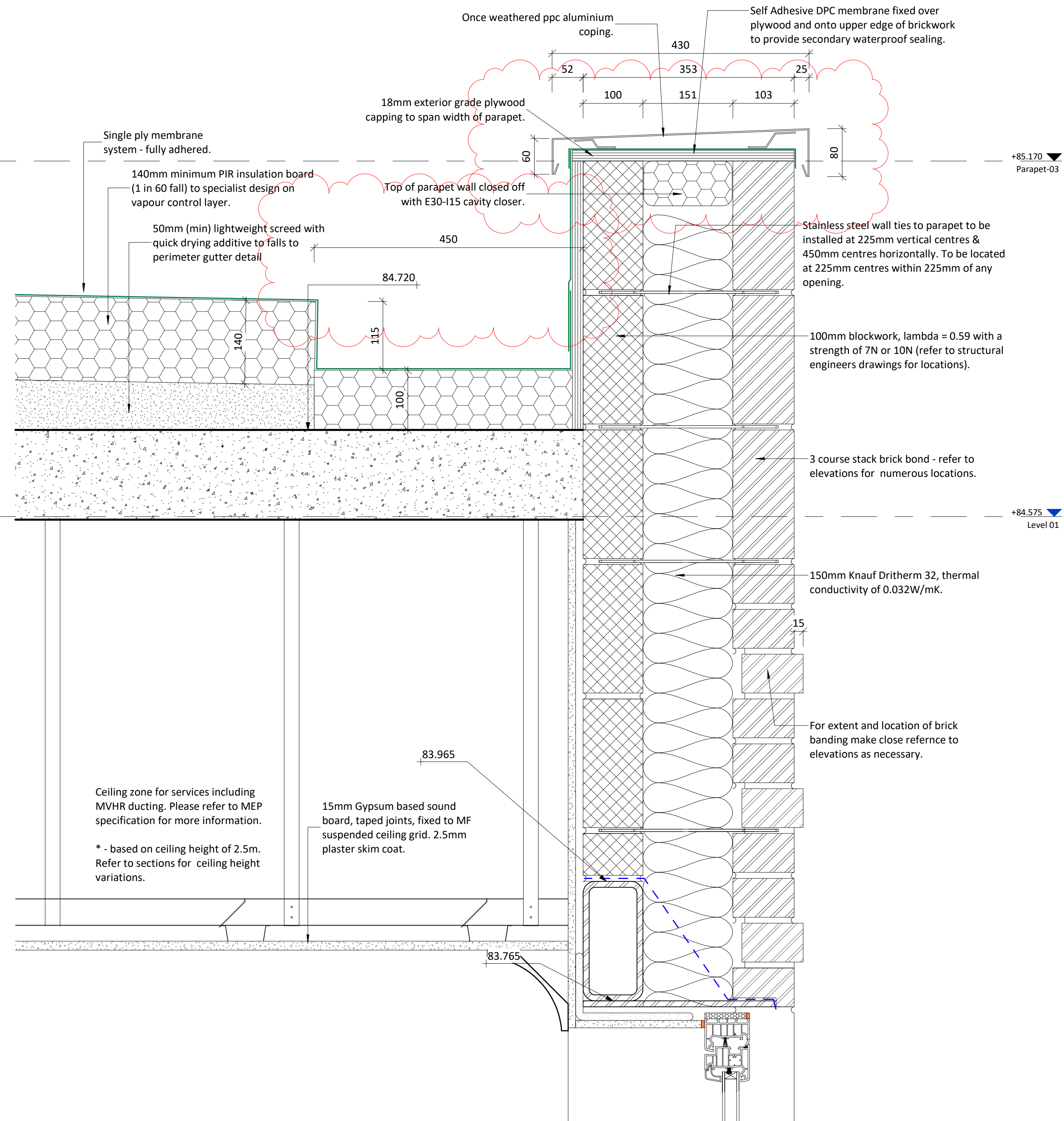
2 Typical Lower Flat Roof - Parapet Detail 1:5
