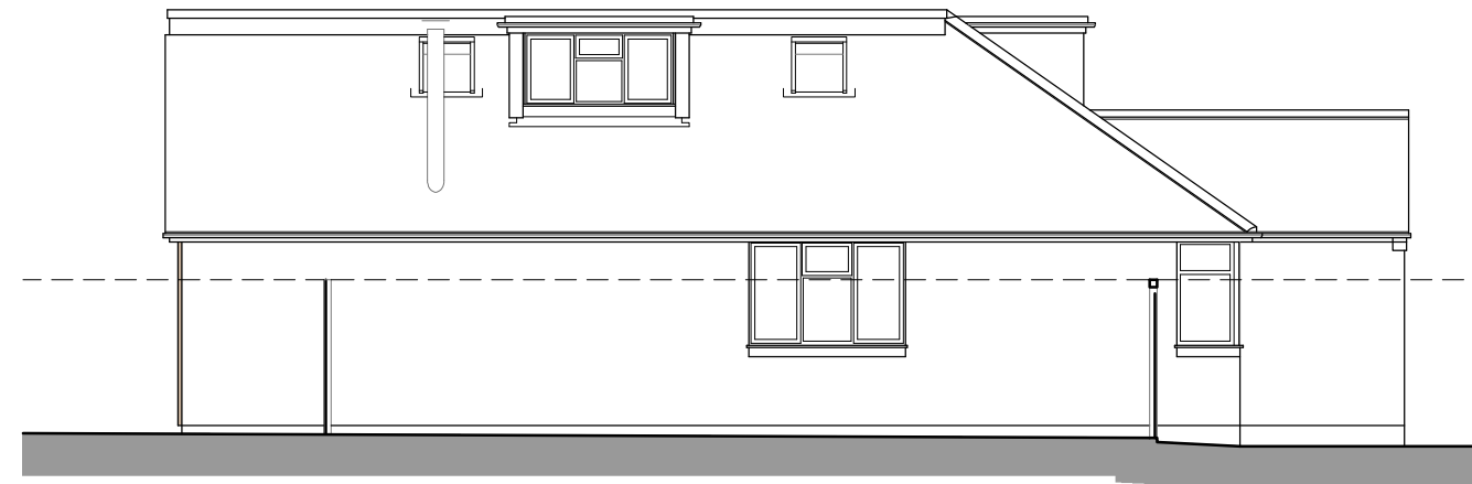
SIDE ELEVATION
