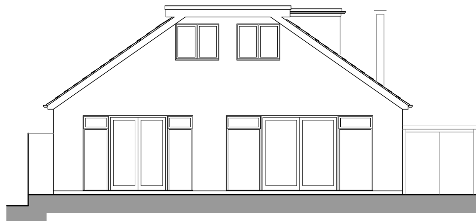
REAR ELEVATION
