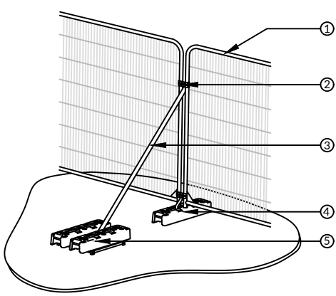
Figure 1: Example of a protective barrier
