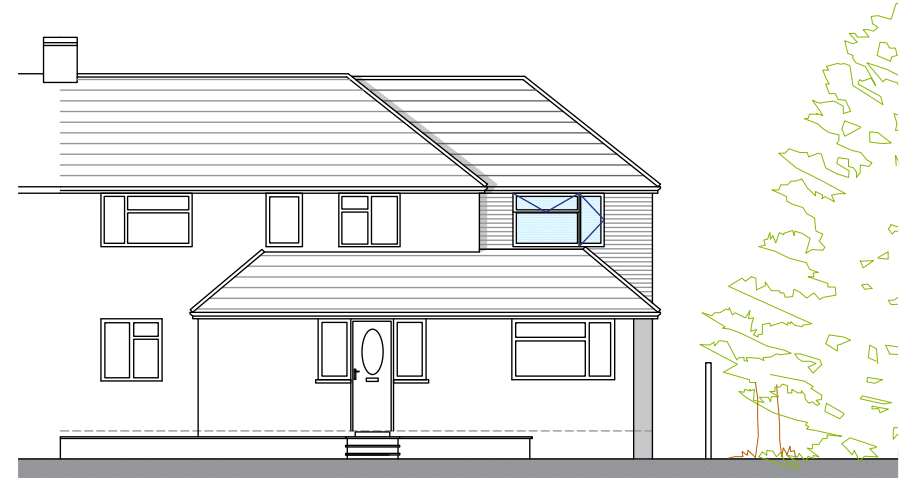
Proposed Front Elevation 1:100 @ A3
