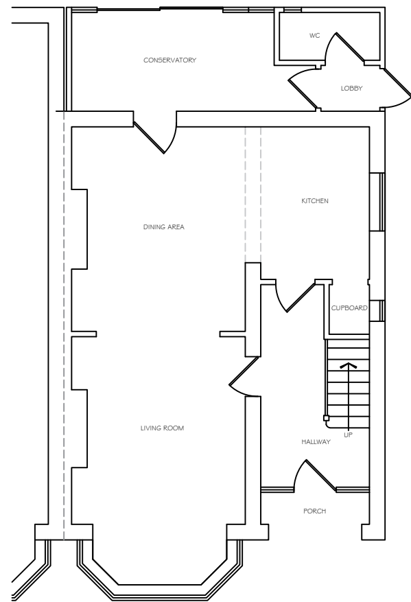
Existing Ground Floor Plan 1:100 @ A3
