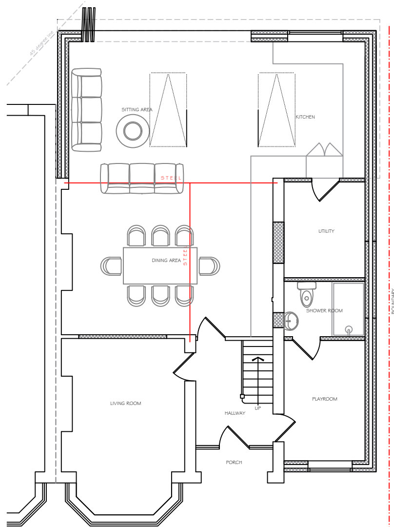
Proposed Ground Floor Plan 1:100 @ A3
