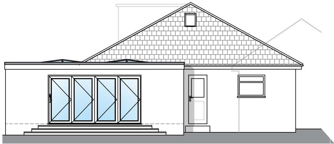
Proposed Rear Elevation 1:100@ A3
