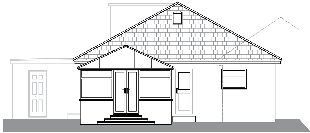
Existing Rear Elevation 1:100@ A3
