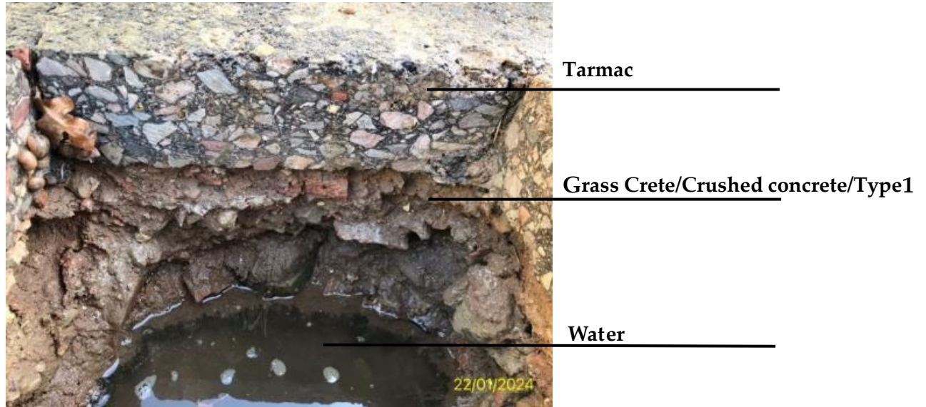
Image 2: Trial Hole 1 – tarmac layer and below this was a single layer of stone hardcore, the geotextile membrane is visible in this photo just below the waterline.
