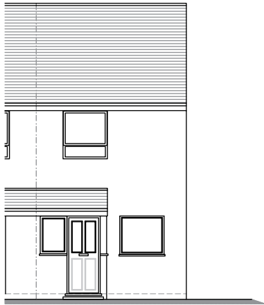
Existing Front Elevation 1:100 @ A3
