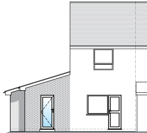
Proposed Rear Elevation 1:100 @ A3
