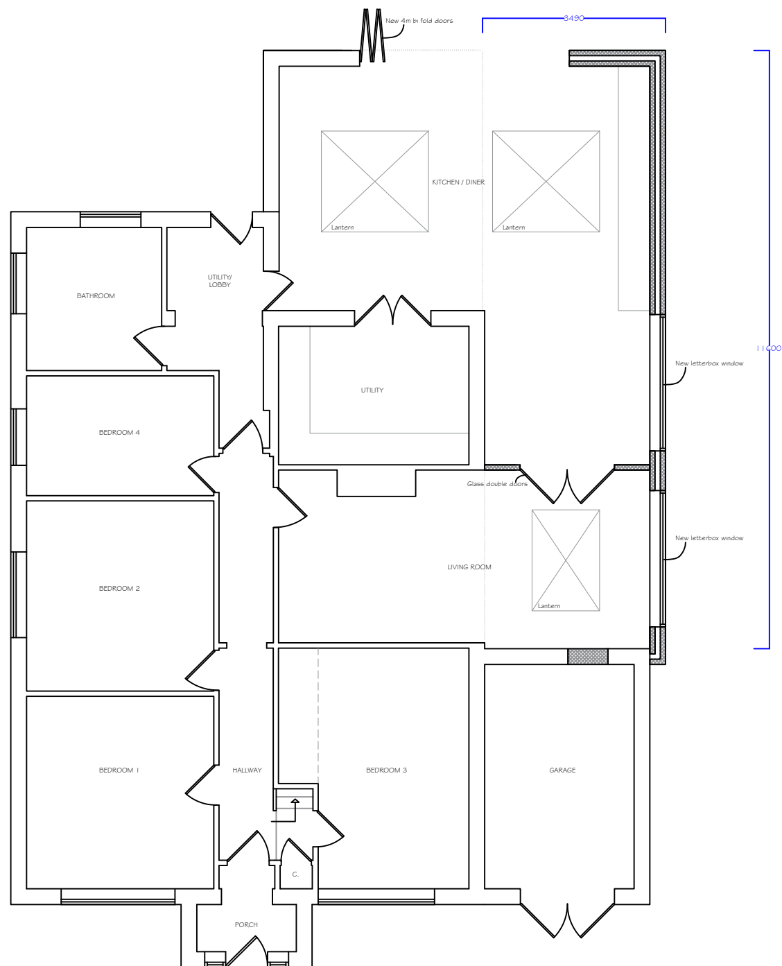
Proposed Floor Plan 1:100 @ A3
