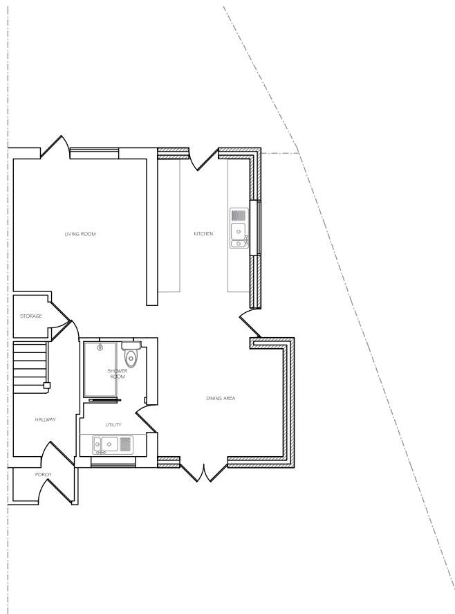
Proposed Ground Floor Plan 1:100 @ A3
