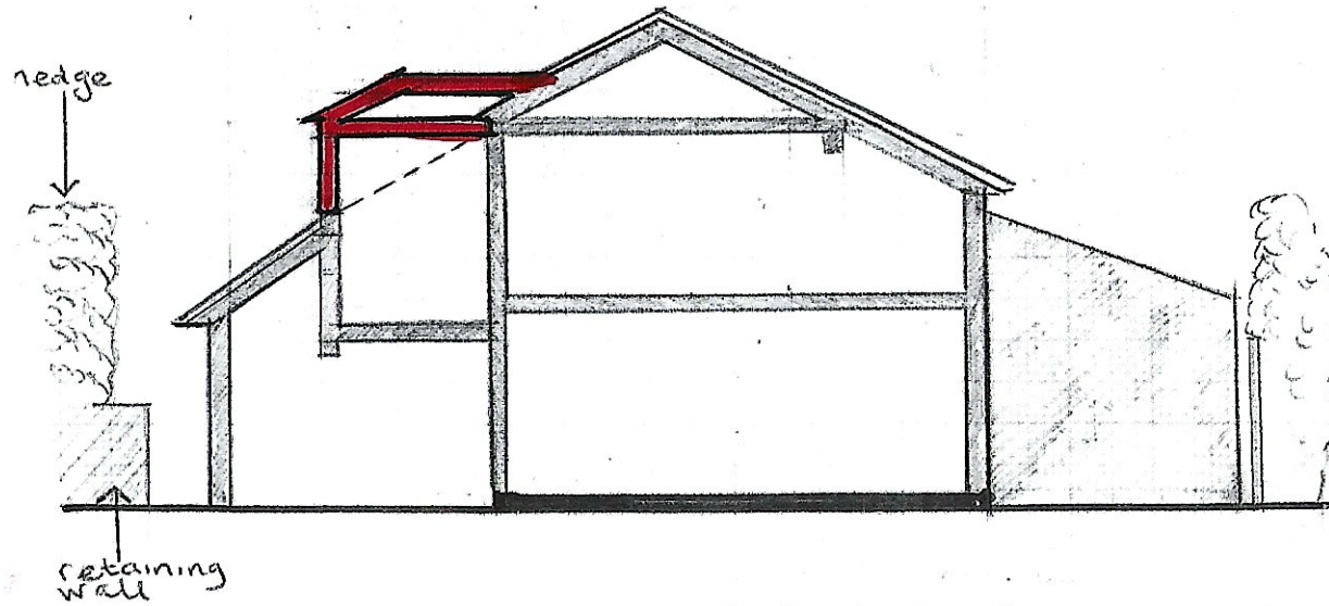
Section plan through proposed rear elevation
