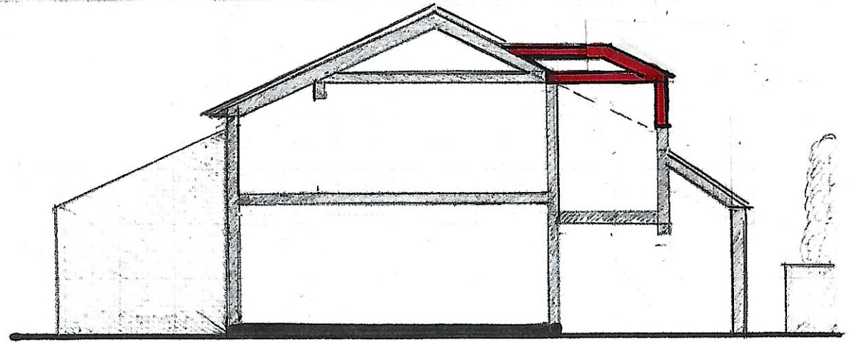
Section plan through proposed front elevation
